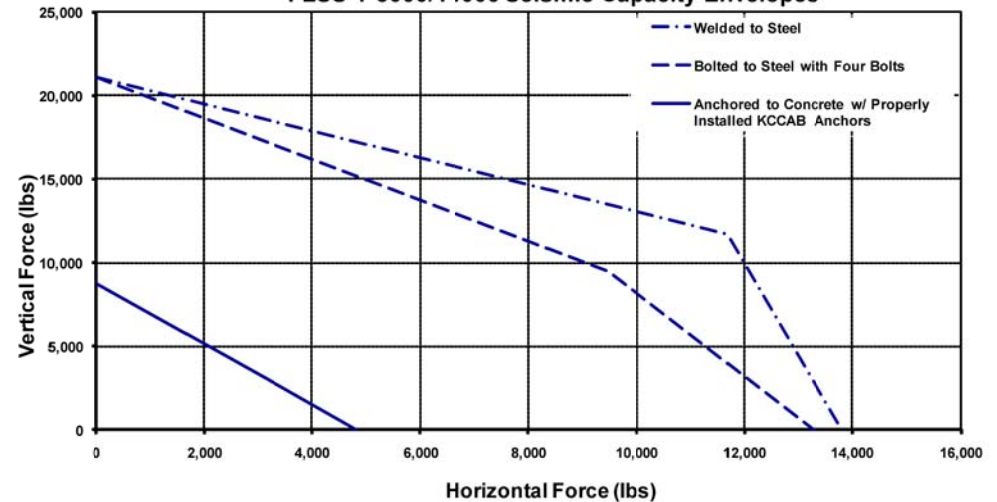
FLSS-1-5000/14000 Seismic Capacity Envelopes
