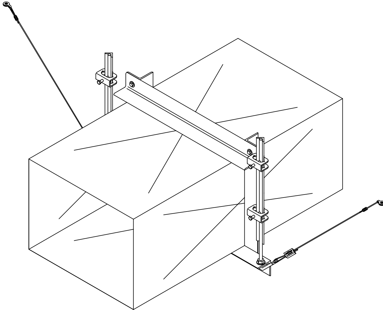
KINETICS MODEL KSCU SEISMIC CABLE RESTRAINT KIT WITH KHRC ROD STIFFENER CLAMPS ASHRAE TYPE J
