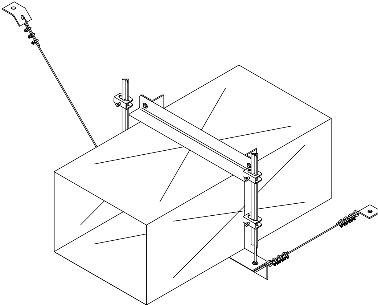
KINETICS MODEL KSCC BULK CABLE RESTRAINT KIT WITH KHRC ROD STIFFENER CLAMPS ASHRAE TYPE J
