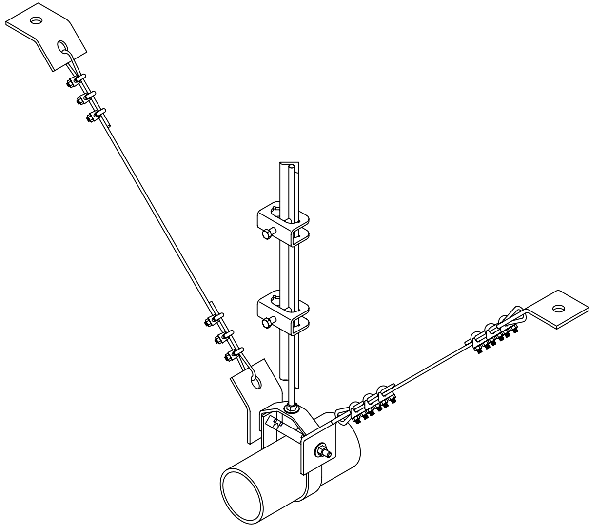
KINETICS MODEL KSCC BULK CABLE RESTRAINT KIT WITH KHRC ROD STIFFENER CLAMPS AND KCHB CLEVIS BRACE ASHRAE TYPE J
