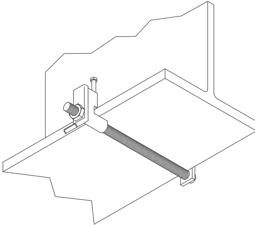
KSBC BEAM CLAMP SEISMICALLY RATED BEAM CLAMP (SHOWN WITH KSCA CLIP)
