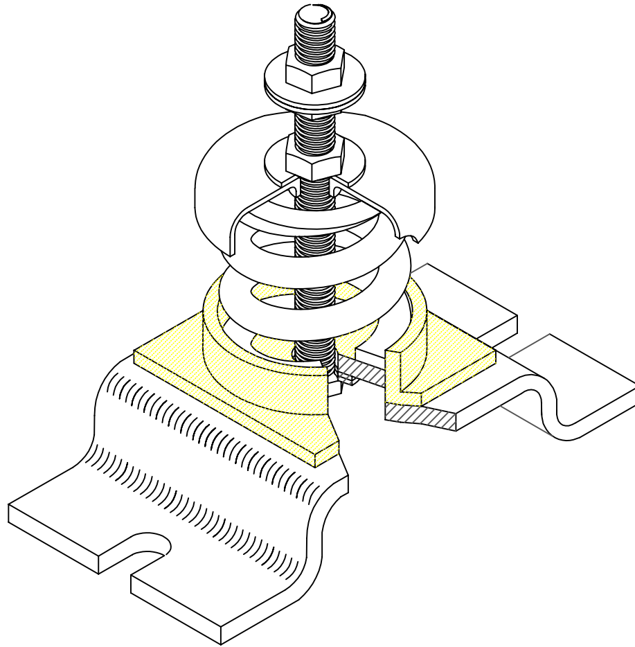
FRS VERTICALLY RESTRAINED ISOLATOR ASHRAE TYPE 3
