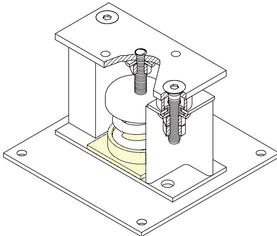
FLS ISOLATOR WITH OPTIONAL OVERSIZED BASEPLATE ASHRAE TYPE 4
