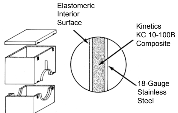
Kinetics Pressure Regulator Enclosure
