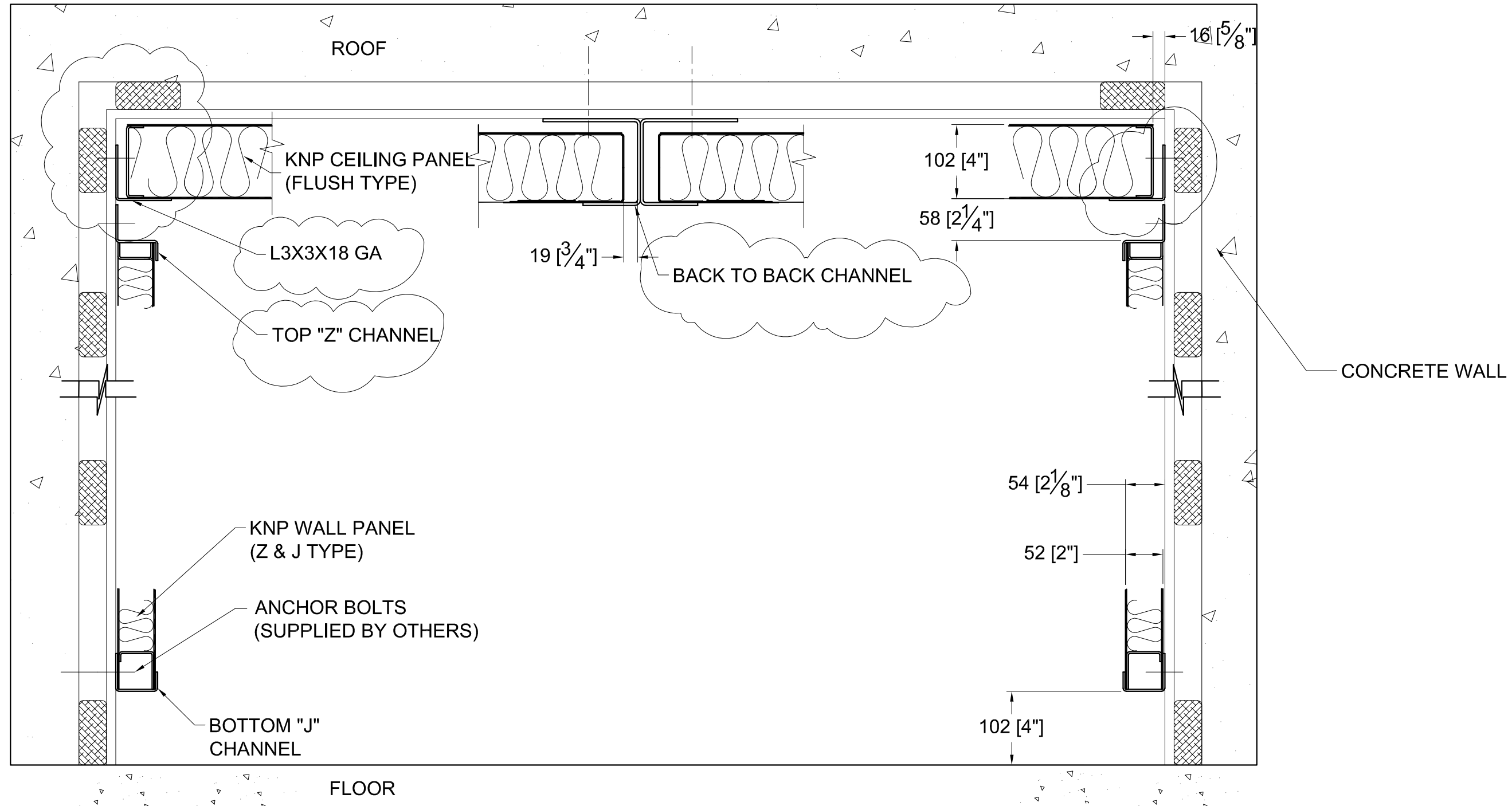
TYPICAL VERTICAL SECTION
