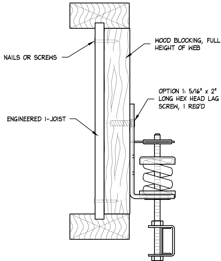
ATTACH NOMINAL 2" x 4" WOOD BLOCKING (OPTION #1)
